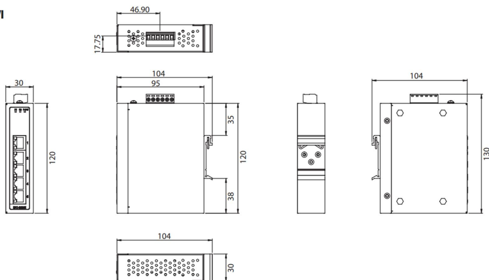
Panel Cut-out Dimensions: 30 x 120 x 95 mm (1.18" x 4.72" x 3.74")
